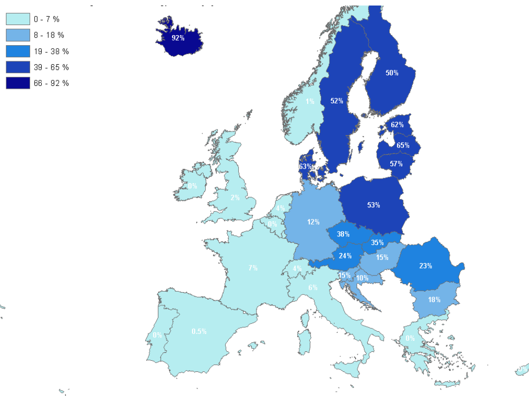
Figure 56: Percentage of the population served by district heating in 2013
