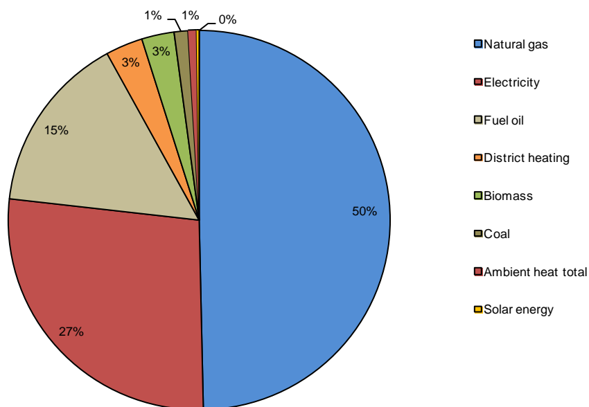
Figure 47 Fuel shares to cover final energy demand for heating and cooling in the services sector
