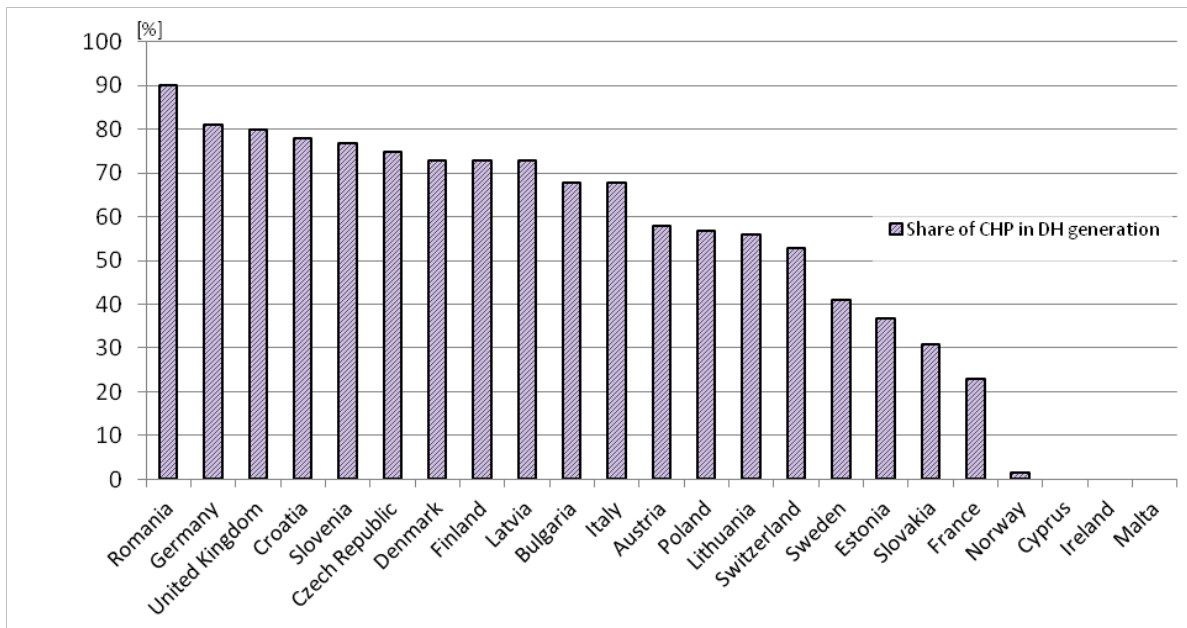
Figure 58: Share of CHP in district heating generation in 2013
