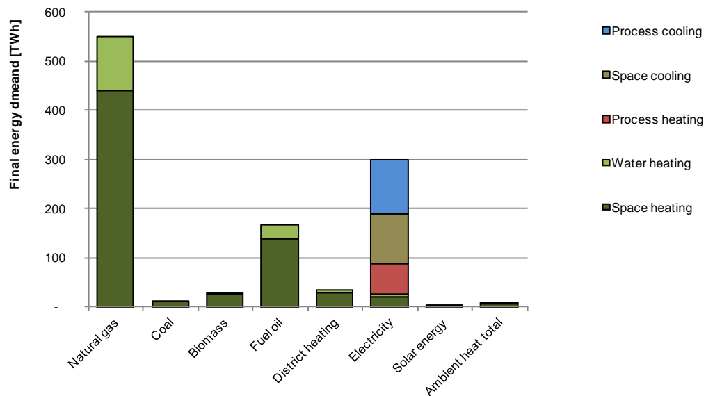
Figure 50 Final energy demand per fuel type and end use in [TWh] for H/C in the services sector
