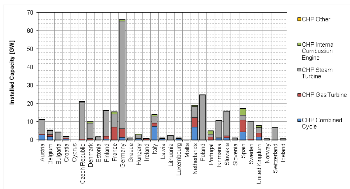
Figure 69: Thermal capacity of combined heat and power plants in Europe.
