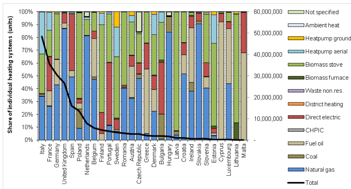
Figure 84: Share of heating technologies and total installed units by country (EU-28).
