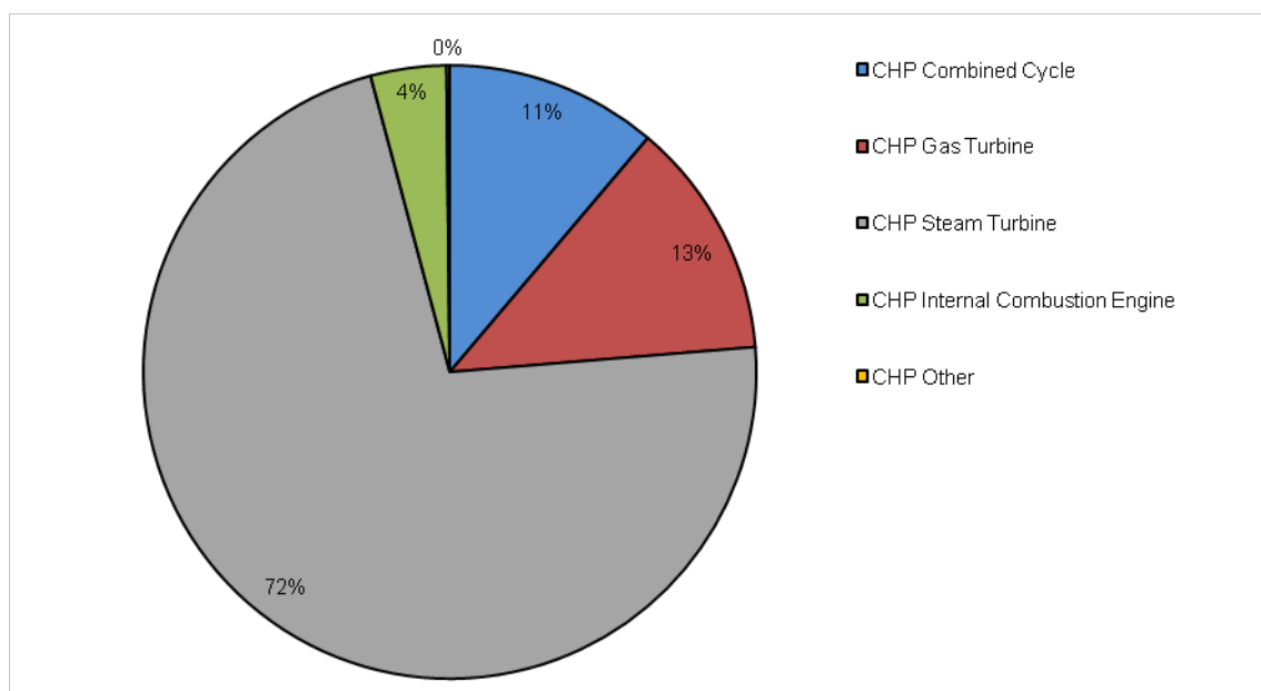
Figure 68: Installed thermal capacity of CHP plants (> 1 MWth) in the EU28 in 2012.
