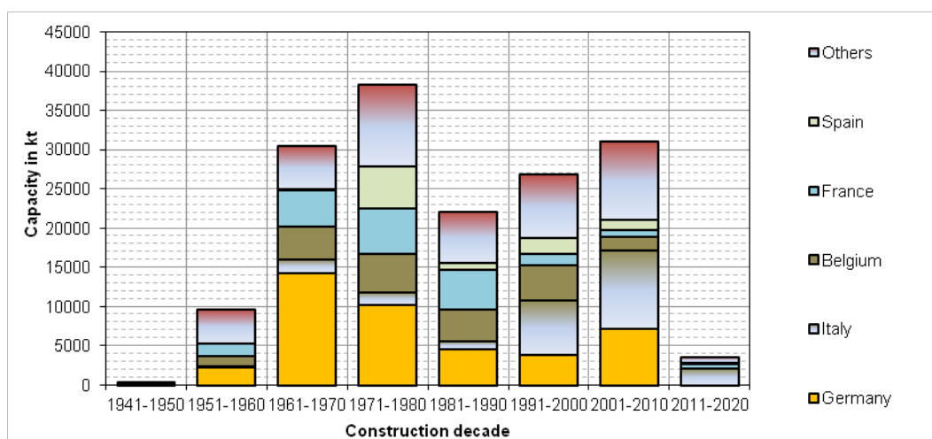
Figure 43: Finished products plant age distribution in kt.
