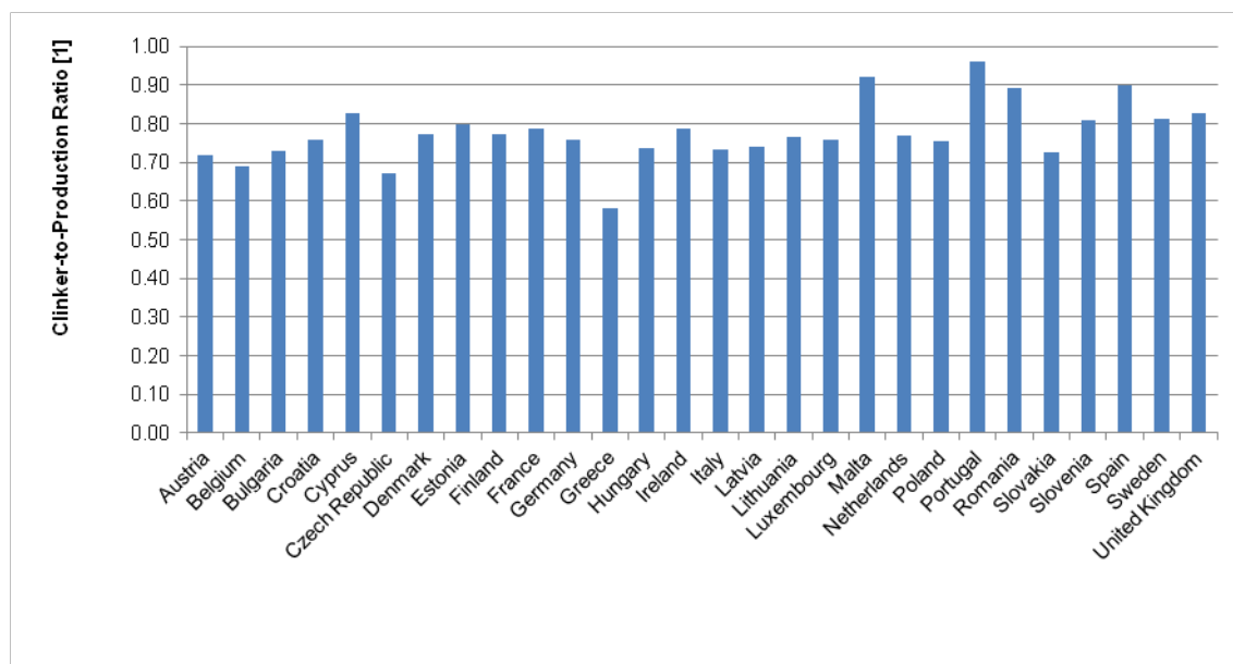
Figure 52: Clinker-to-production ratio (Clinker production divided by cement production) of the EU28 countries in 2010.
