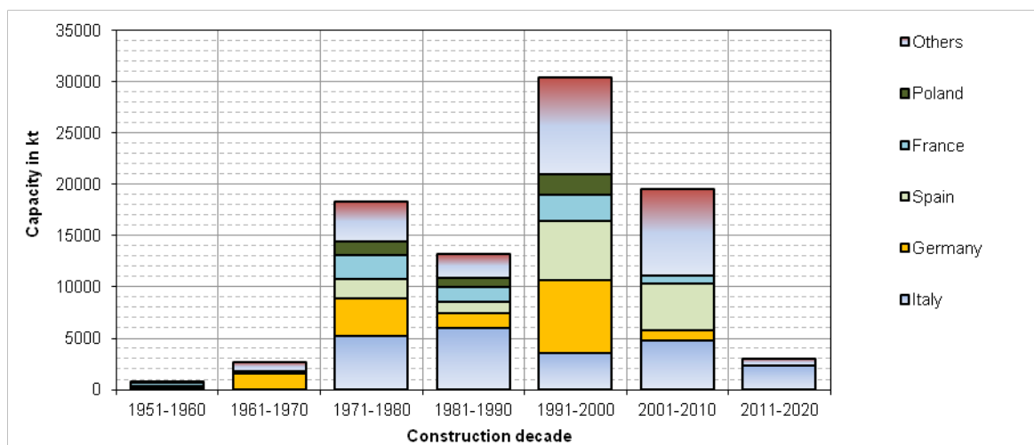
Figure 32: Plant capacity age distribution EAF in kt.
