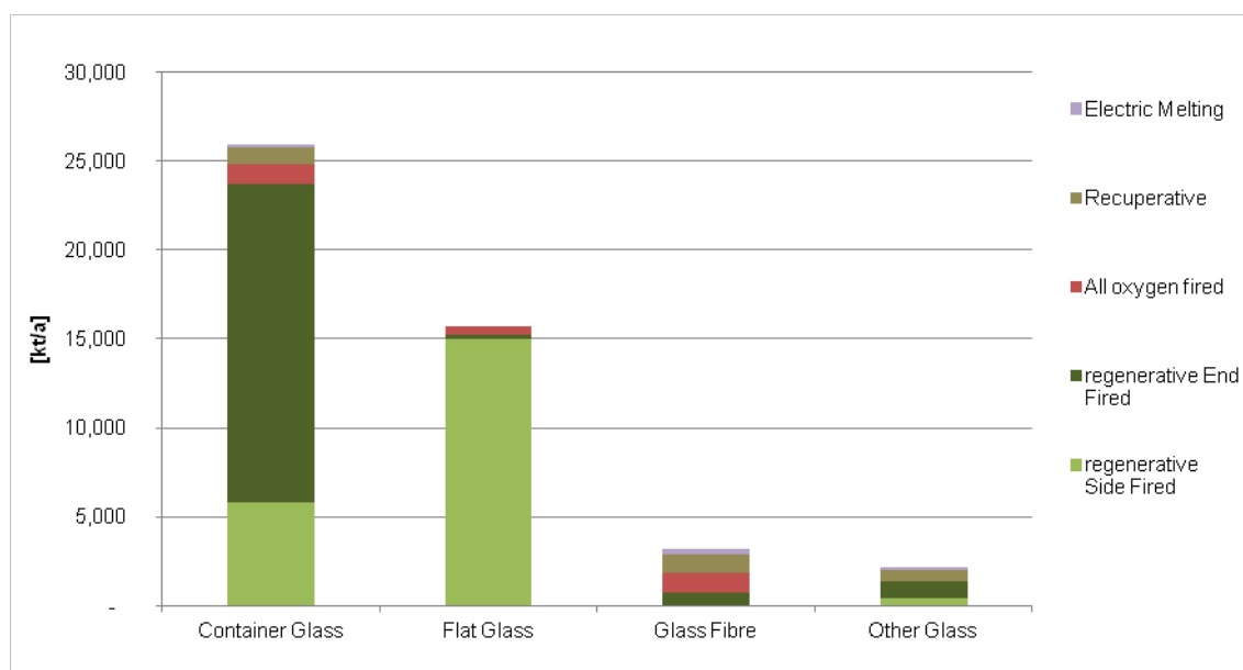
Figure 56: Technologies used in the different Glass sectors the EU 28 and Norway, Switzerland and Iceland; Capacities in [kt/a].
