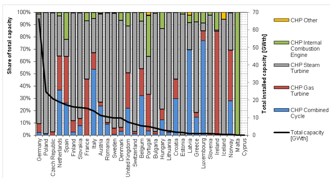
Figure 70: Relative portion of thermal capacity of combined heat and power plants in Europe.
