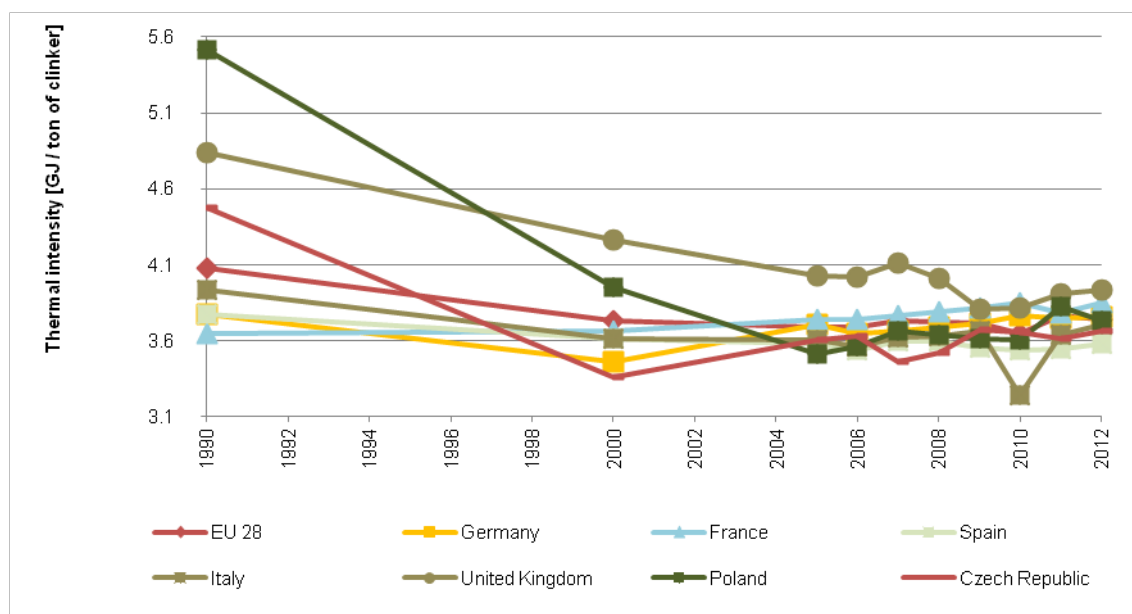
Figure 46: Thermal energy intensity in GJ per ton clinker for the EU 28 and main cement producing countries in Europe.
