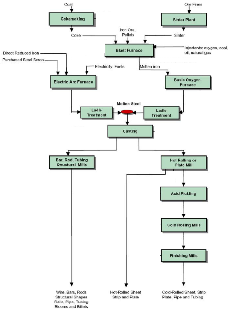
Figure 29: Steel production routes.
