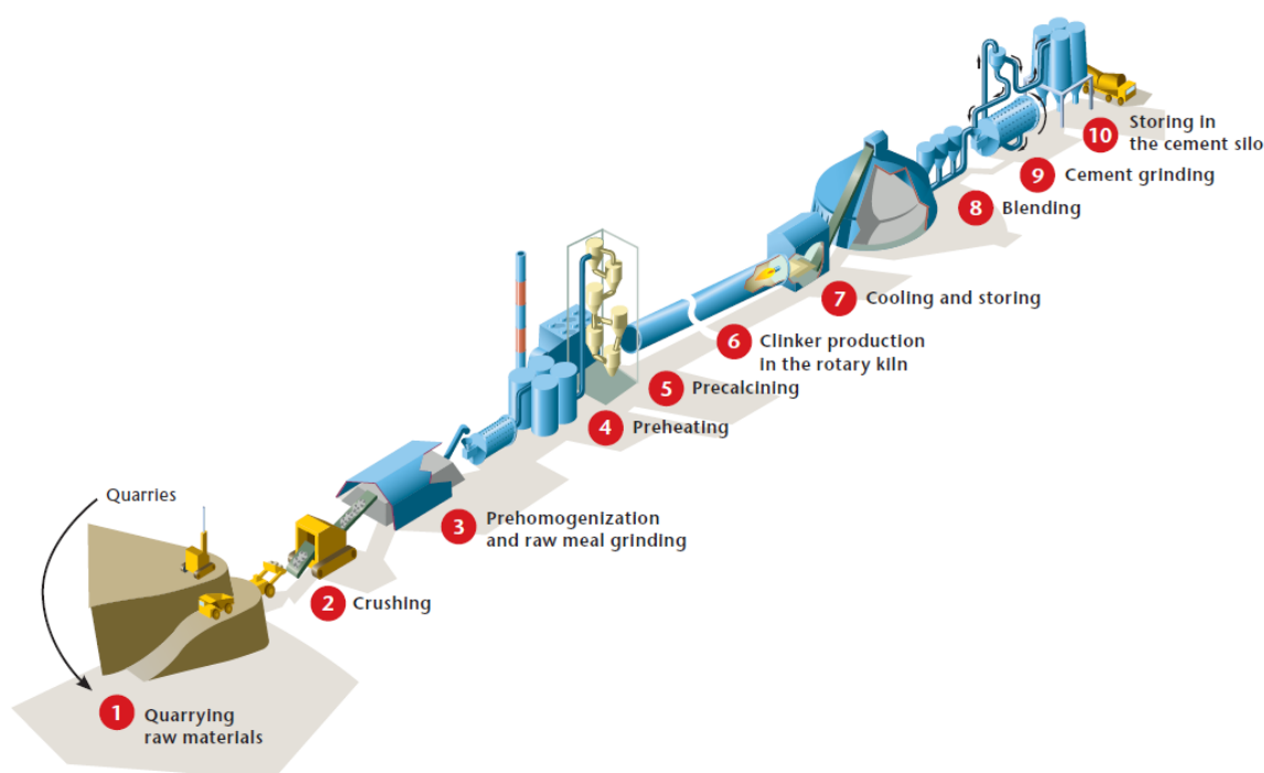
Figure 45: Industrial process of cement manufacturing.
