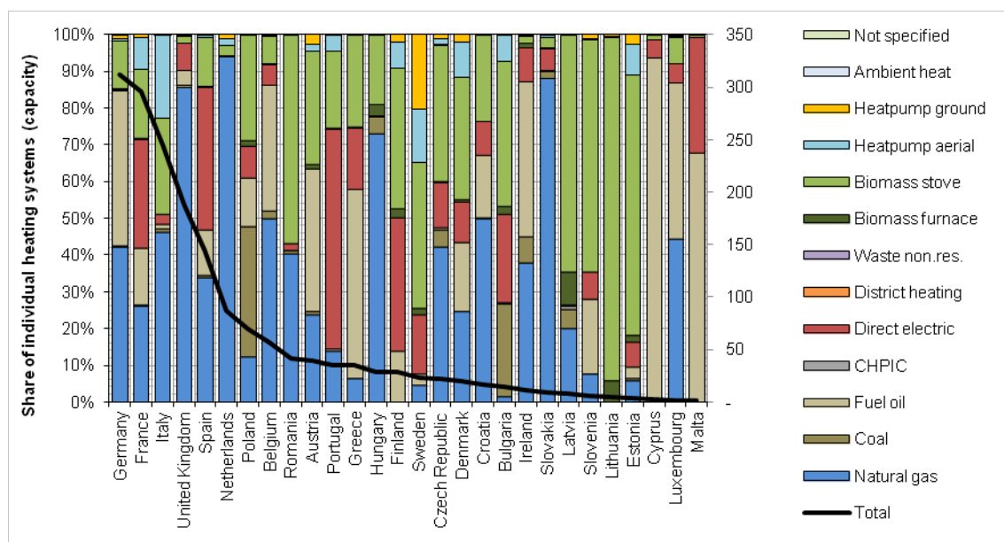
Figure 83: Share of heating technologies and total installed capacity by country (EU-28).
