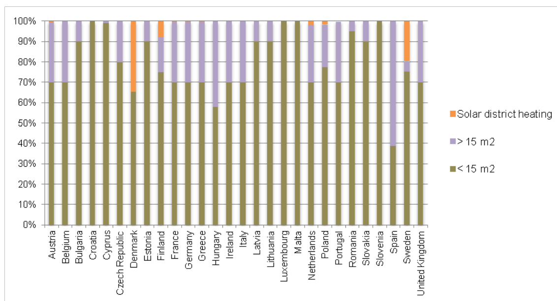
Figure 17: Size distribution of flat plate collectors in Europe in 2012
