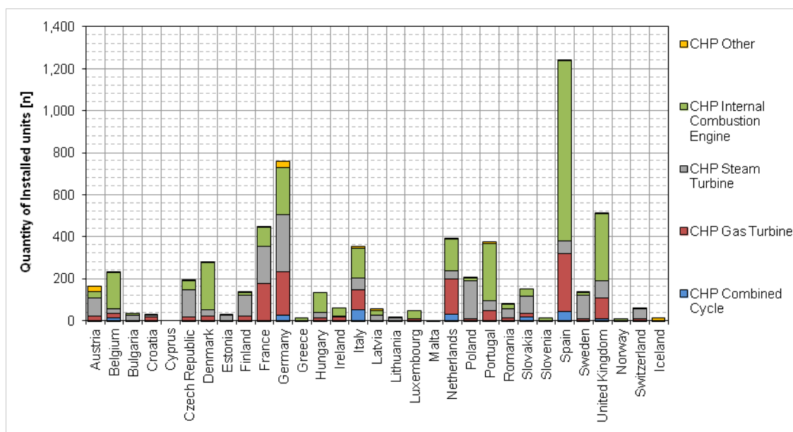
Figure 72: Stock (quantity) of combined heat and power plants in Europe in 2012
