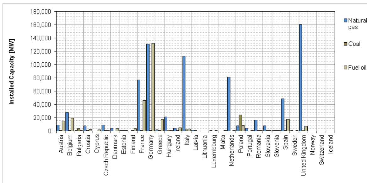
Figure 9: Installed capacity in MW th of natural gas, oil and coal boilers by country.
