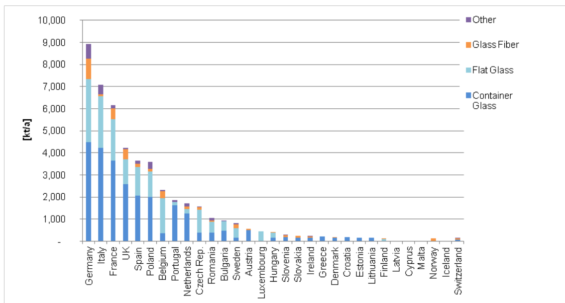
Figure 57: Installed capacities [kt/a] by country divided by production sectors in 2012.
