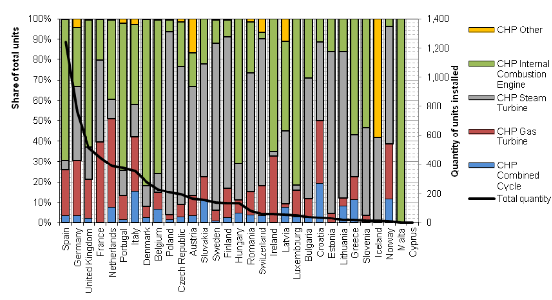
Figure 73: Relative portion of technologies in the stock of combined heat and power plants in Europe.
