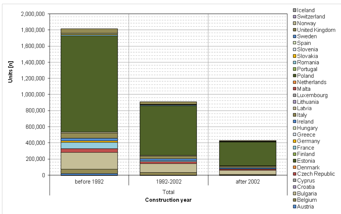
Figure 8: Age distribution of installed units of coal fired boilers in Europe.
