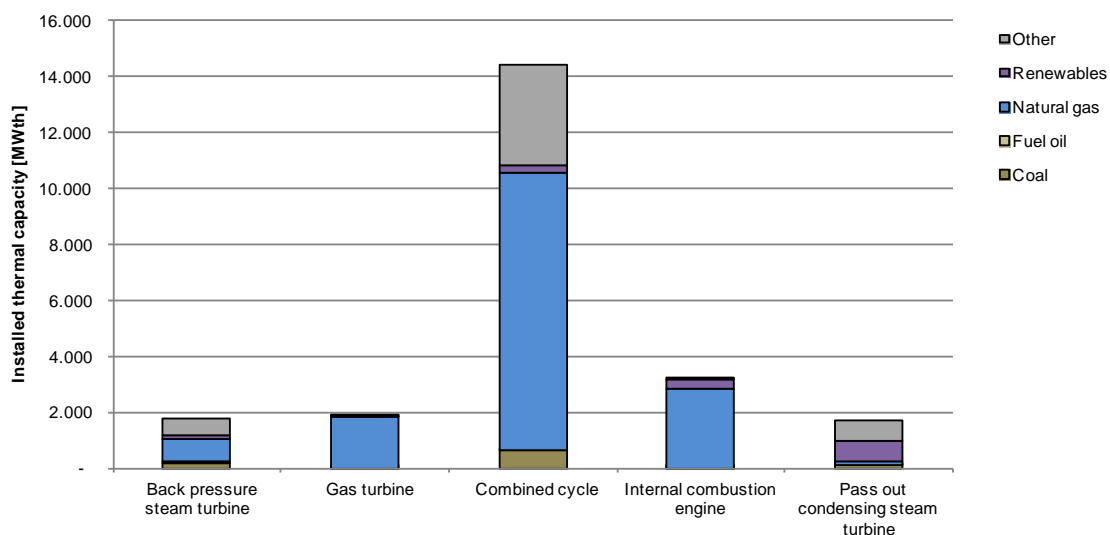
Figure 28: CHP thermal capacity by fuel type and technology in the UK in 2013 (source: Department of Energy and Climate Change 2015a)
