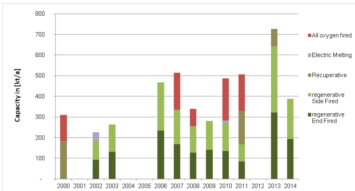
Figure 59: New furnace capacities in container glass industries since 2000 [kt/a] in EU28 and Norway, Switzerland and Iceland.
