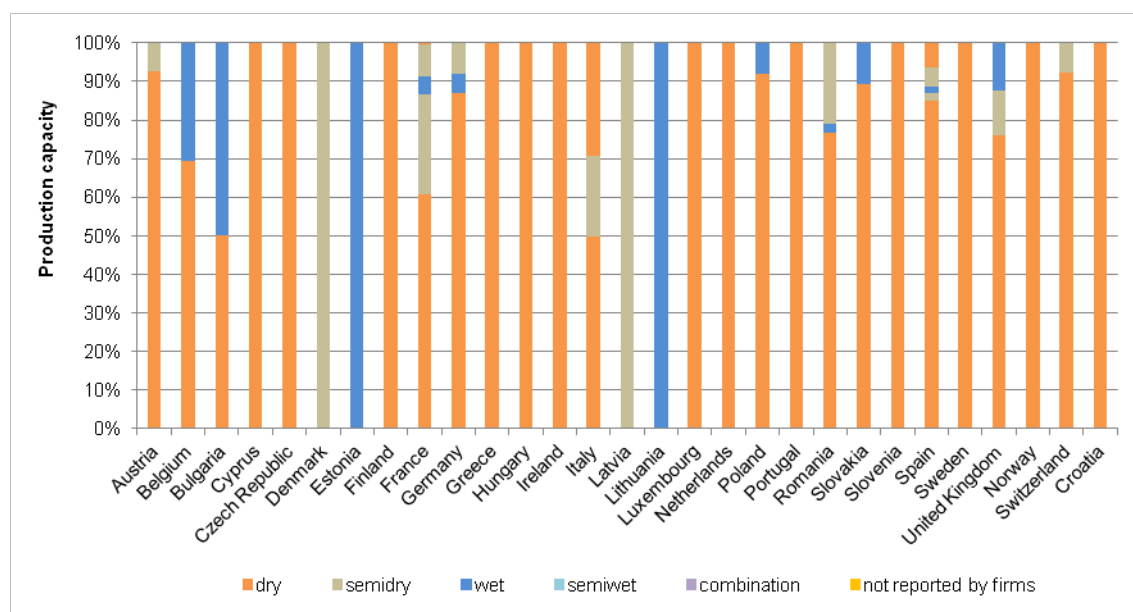
Figure 49: Type of kiln installed in 2012 based on production capacity.
