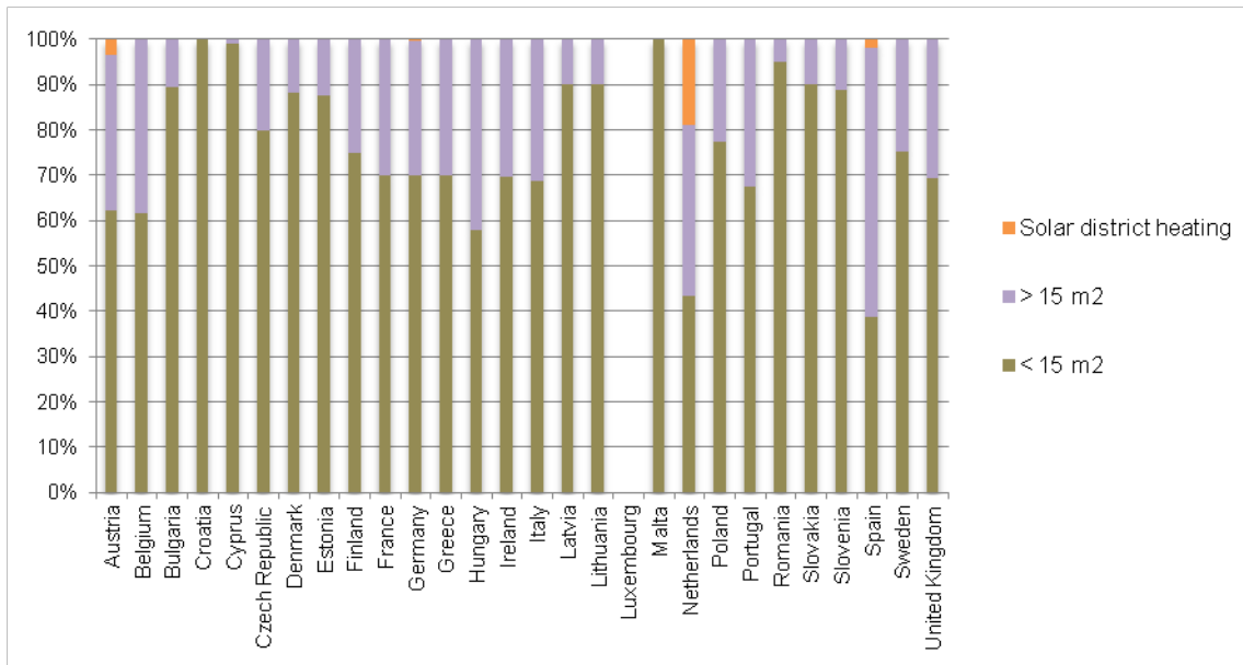
Figure 18: Size distribution of vacuum collectors in Europe in 2012
