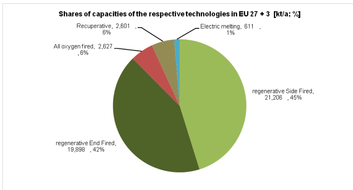
Figure 55: Shares of capacities of the respective technologies in EU28 and Norway, Switzerland and Iceland [kt/a; %].
