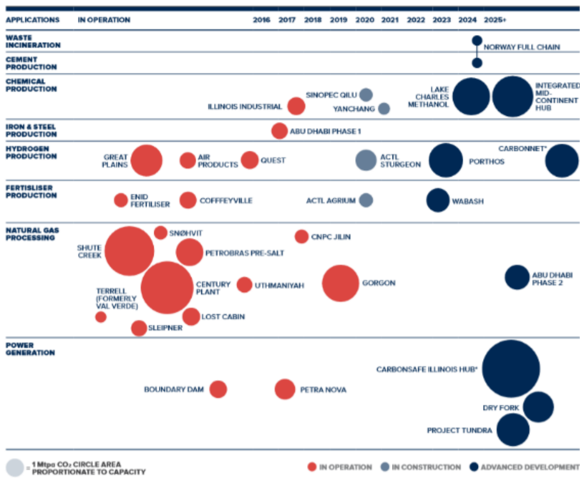
Source 56 Global status of CCS 2019, Report of the Global CCS Institute
