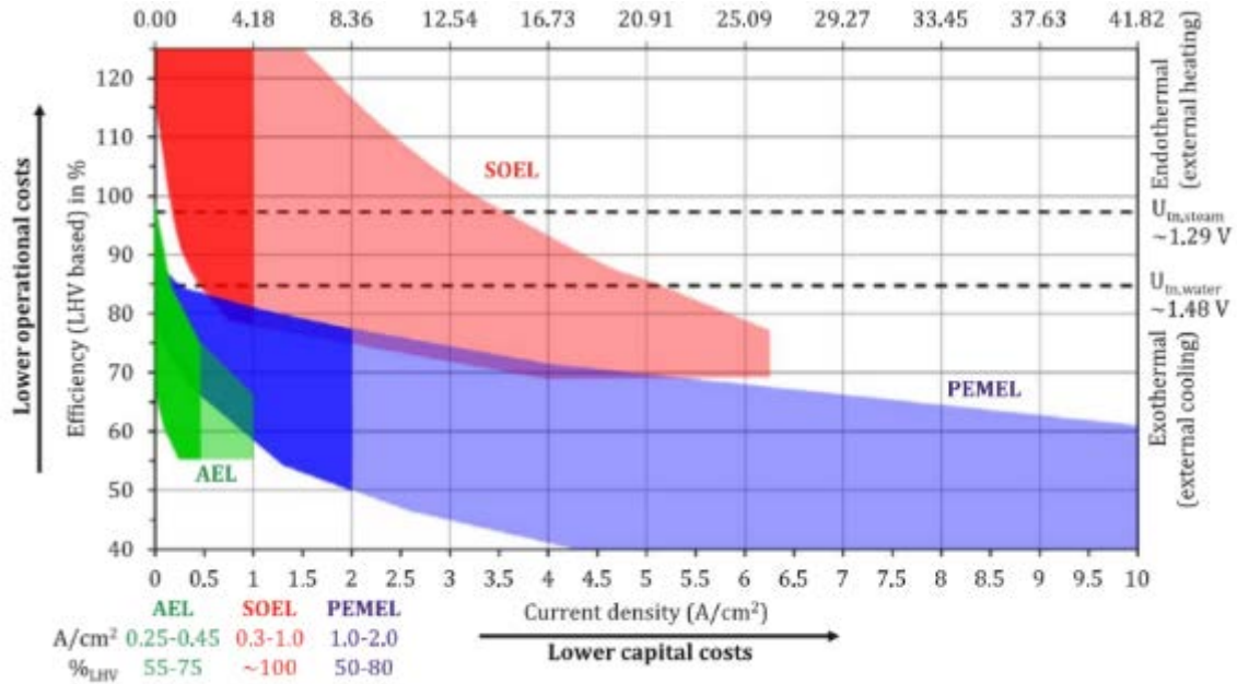
Figure 5 Specific Hydrogen Production per Cell Area
