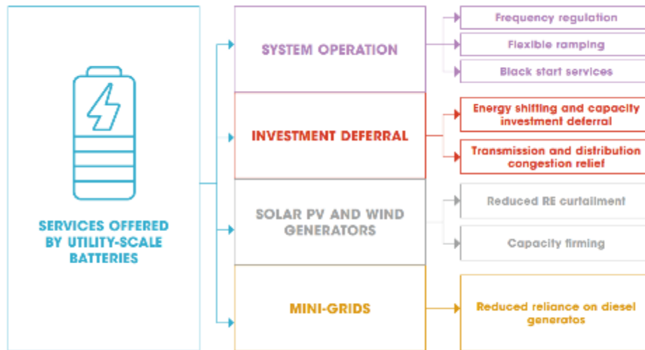
Figure 12 Summary of services that can be provided by Energy Storage in the Power System
