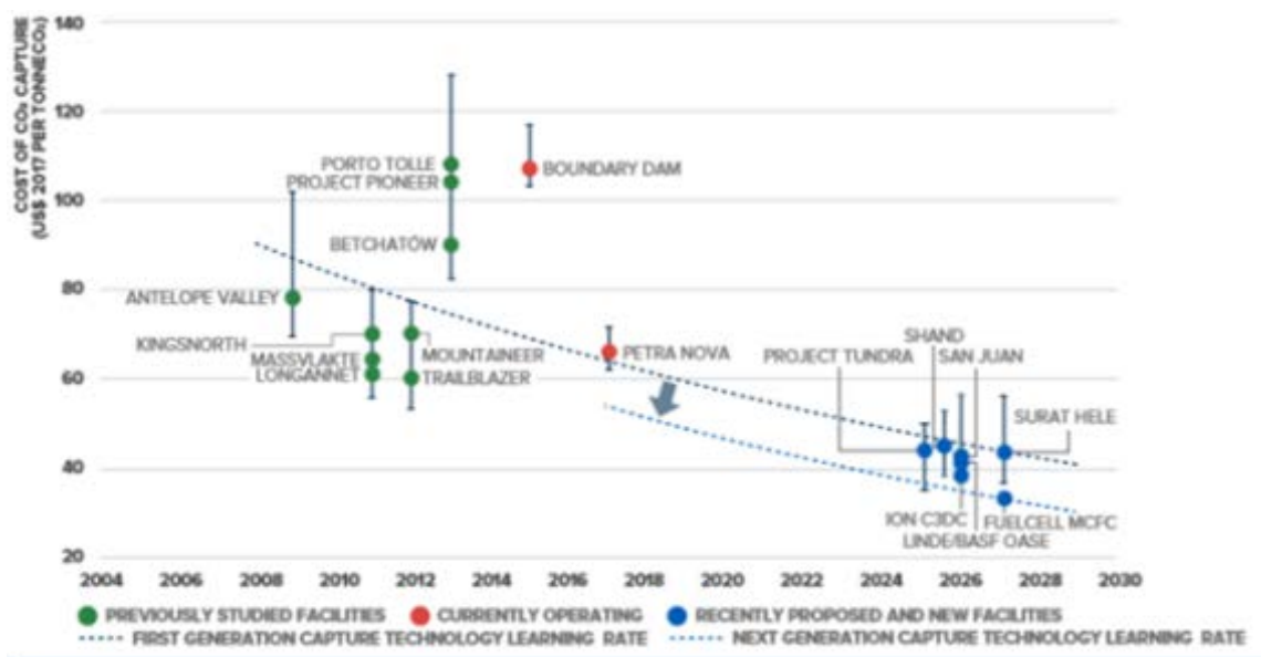
Figure 57 Levelised cost of CO 2 capture for large-scale post-combustion facilities at coal-fired power plants, including previously studied facilities
