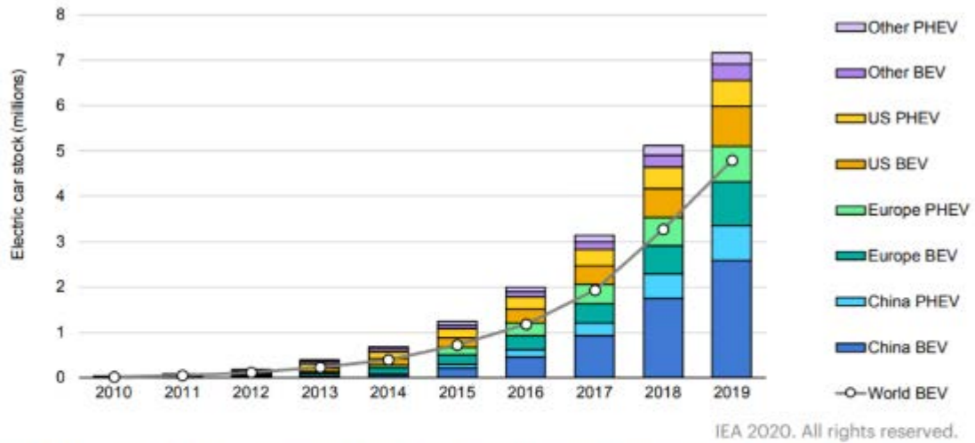
Figure 14 Global Electric Vehicles and Plug in hybrid car stock, 2010-2019
