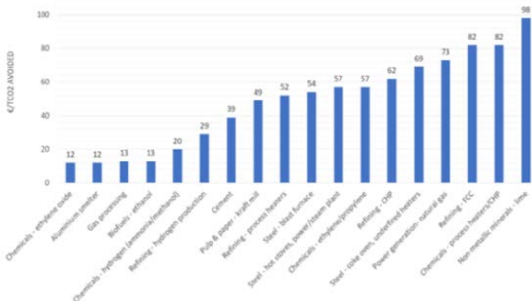
Figure 55 Overview of median carbon capture costs in various industrial processes
