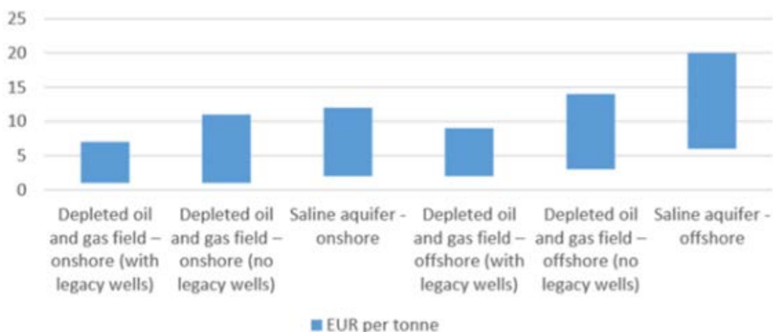
Figure 56 Storage costs in the EU28 per formation type
