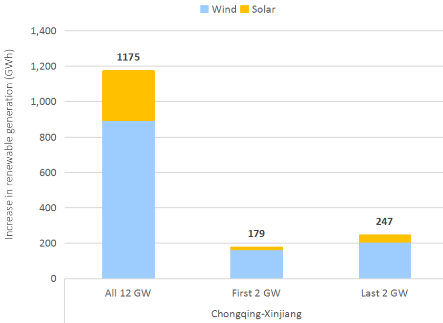
Figure 9.9: Increase in renewable electricity generation for the full project, the first 2 GW and the last 2 GW of the Chongqing-Xinjiang line in GWh/yr. The increase is due to the reduction in curtailment of wind and PV.
