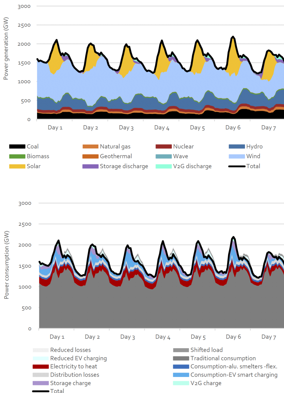
Figure 5.7: Profiles for power generation (top) and consumption (bottom) in China in winter 2050 (Below 2°C Scenario).
