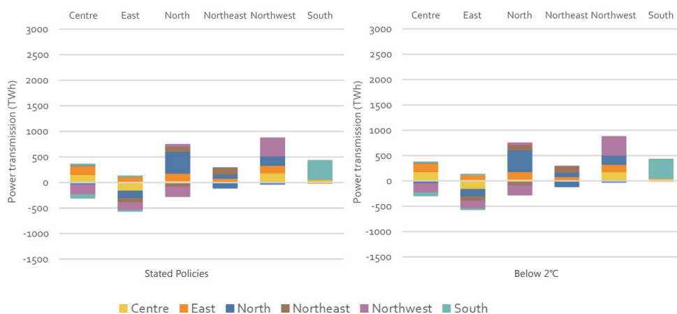
Figure 5.9: Power transmission between regions in 2050.
