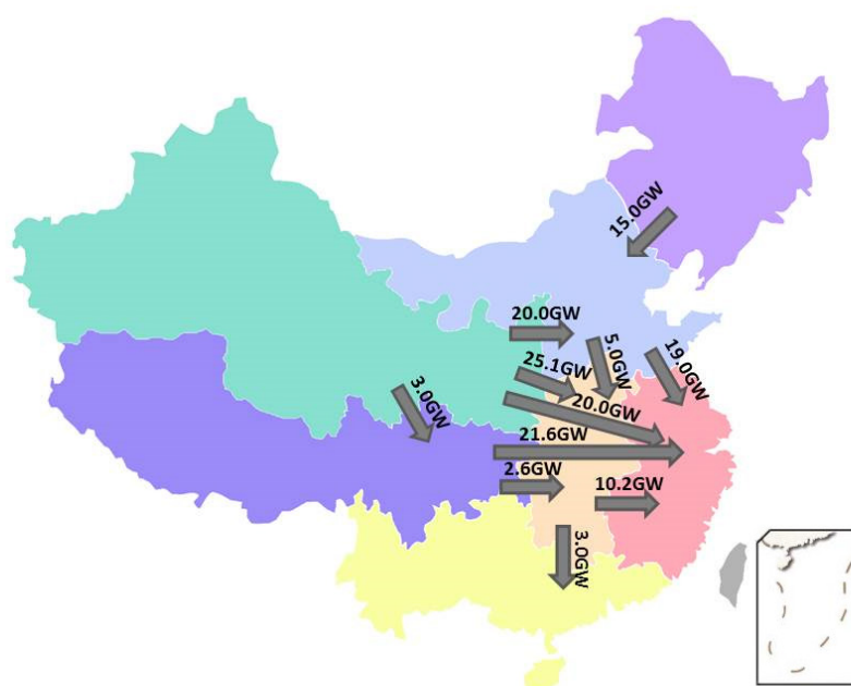
Figure 7.1: SGERI model footprint and capacities between model areas (regions), 2020.
