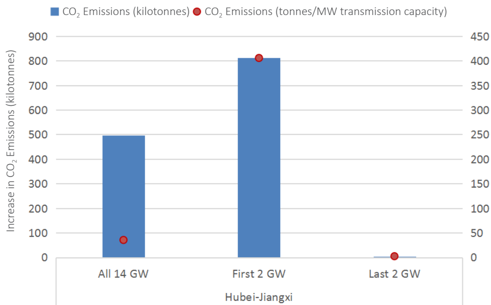
Figure 9.2: Increase in CO 2 emission for the full project, the first 2 GW and the last 2 GW of the Hubei-Jiangxi line in kilotons/yr and the respective CO 2 emission change per MW transmission capacity. Positive values show an increase in CO 2 emissions.
