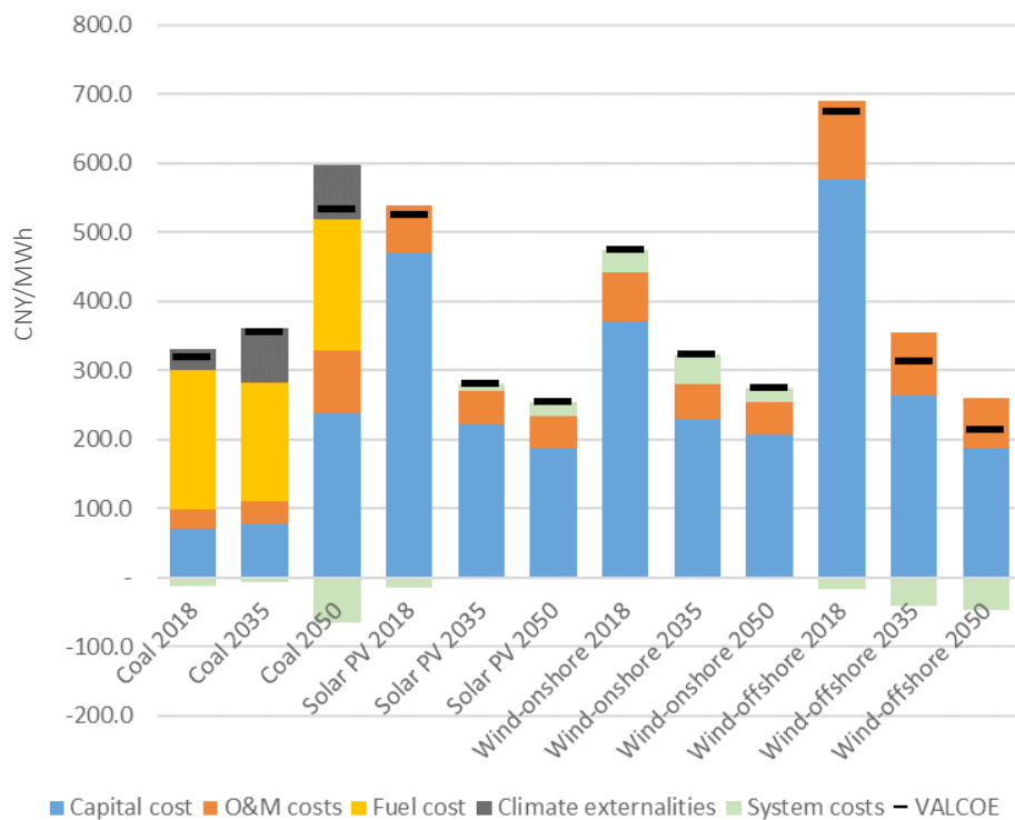
Figure 5.6: Levelised cost of electricity from new coal, wind and solar (utility scale PV) including value adjustments (system costs) and average operating hours from the Stated Policies Scenario.
