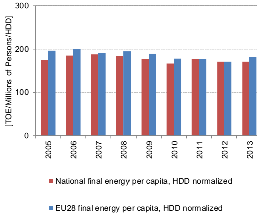
CZ) Residential: final energy consumption per capita, HDD normalized
