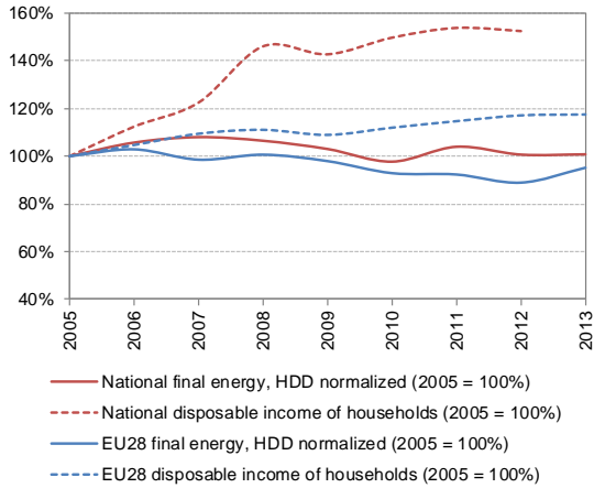
CZ) Residential: final energy consumption, HDD normalized vs disposable income of households
