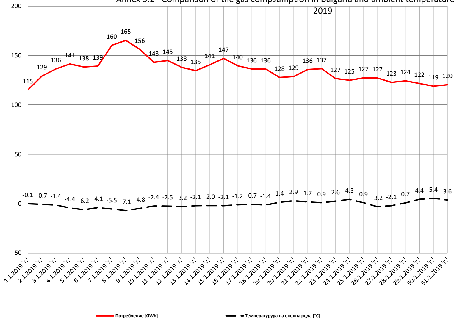
Annex 5.2 - Comparison of the gas compsumption in Bulgaria and ambient temperature (Sofia) for January
