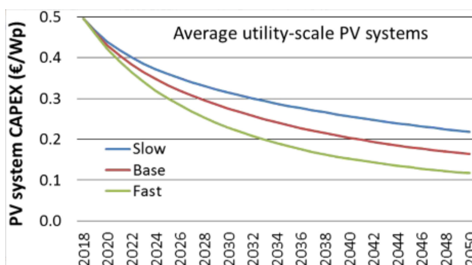
Figure 18 Utility-scale PV capital expenditure (CAPEX) in Europe for the years 2018 to 2050 in three different scenarios (EUR/W)
