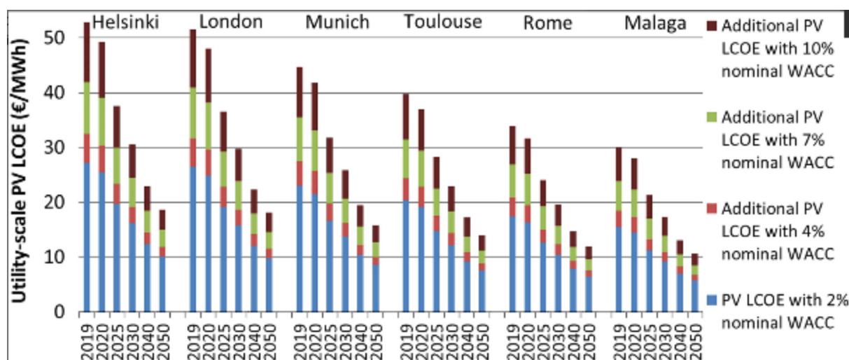
Figure 19 PV LCOE for utility systems in six European locations, years 2019 to 2050 ( EUR 2019/MWh), taxes not included
