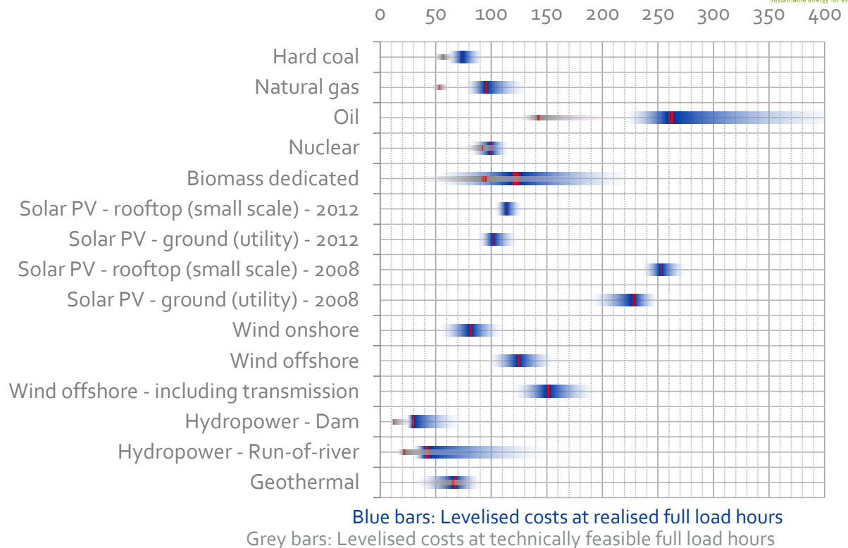
Figure S - 7: Levelised costs of energy in EU28 for electricity (in €2012/MWh)
