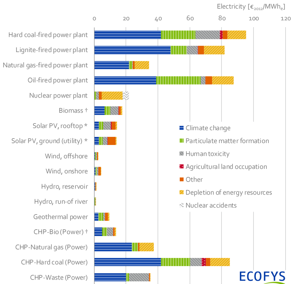
Figure 3-8: External costs per technology for electricity technologies, EU28 weighted averages (in \text{€}_{2012}/\text{MWh}_e ).
