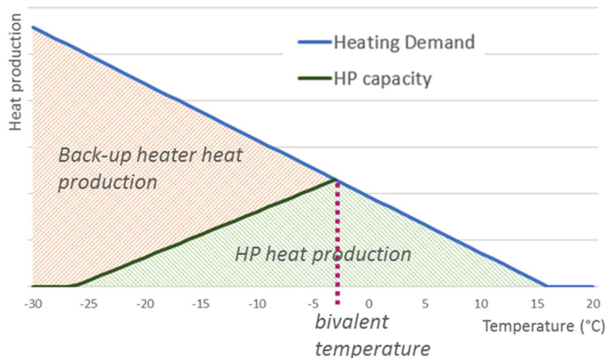
Figure 5 - Decomposition of the heat production between the (air-source) heat pump and the back-up heater in function of the outdoor temperature (i.e. temperature of the heat source)
