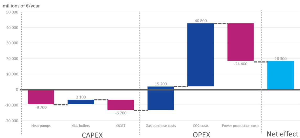
Figure 21 – Economic benefits of option A vs option 0 the EUCO30-2050 scenario
