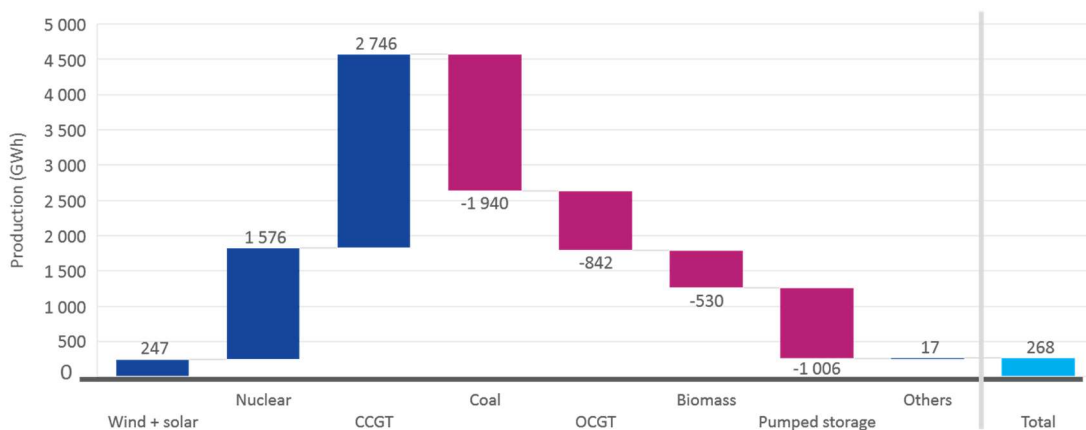
Figure 25 - Power production in scenario REF16-2030 (Option B vs Option A)
