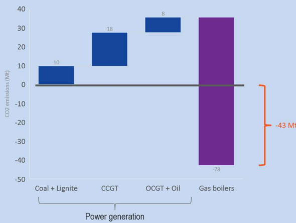
Figure 22 - CO 2 emissions in scenario EU30-2050 scenario (Option A vs Option 0)
