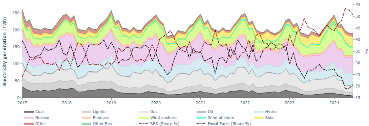
Figure 13 – Monthly electricity generation mix in the EU
