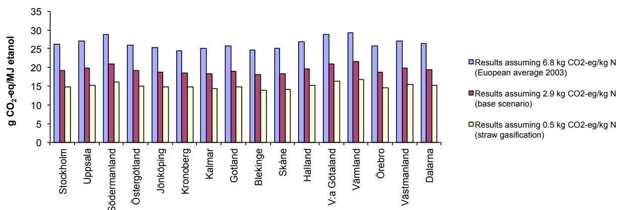
Figure 8. Greenhouse gas emissions (g CO 2 -eq/MJ ethanol) for winter wheat, cultivated with nitrogen fertilizers produced by various production methods. Nitrogen fertilizers produced with best available technology are values used in the base scenarios, which are compared in the diagram with values for European average production and the more futuristic option of straw gasification.
