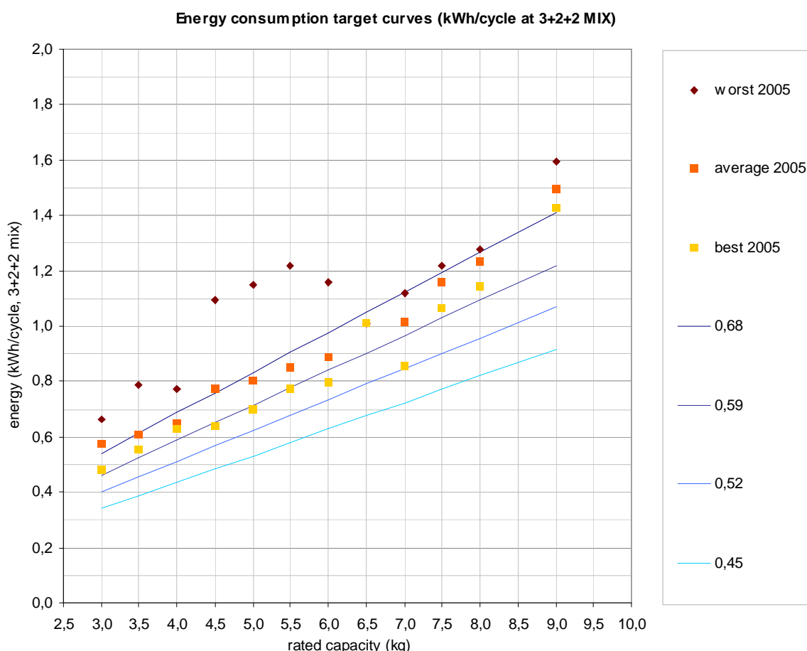
Figure 8: Indicative energy consumption per cycle for the proposed energy efficiency requirements stage 1 and 2 compared to current class A thresholds
