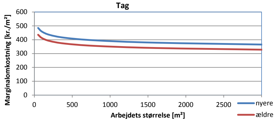
Figure 8. Marginal cost of post-installation insulation of roofs in connection with the replacement of roof-cladding materials.
