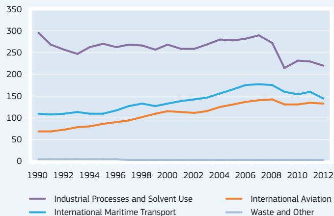
CO 2 Emissions – EU-28 – Other Than Fuel Combustion (Million ton CO 2 )
