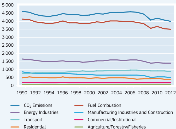
CO 2 Emissions – EU-28 – Total and Fuel Combustion (Million ton CO 2 )
