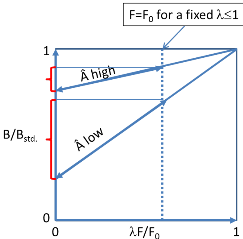
Figure 5-3: Emission of Black Carbon from a biofuel relative to that of kerosene ( B/B_{std} ) as a function of rated thrust ( F/F_0 , i.e. thrust divided by maximum thrust) for alternative fuels with different aromatic contents (normalized to the average aromatic content of kerosene, \hat{A} ). The value of \lambda ( 0 \leq \lambda \leq 1 ) describes how sensitive BC emission depends on thrust setting. The broken vertical line marks full thrust for a fixed value of \lambda < 1 . Read braces on the lhs axis indicate the range of BC emission between no thrust and full thrust.
