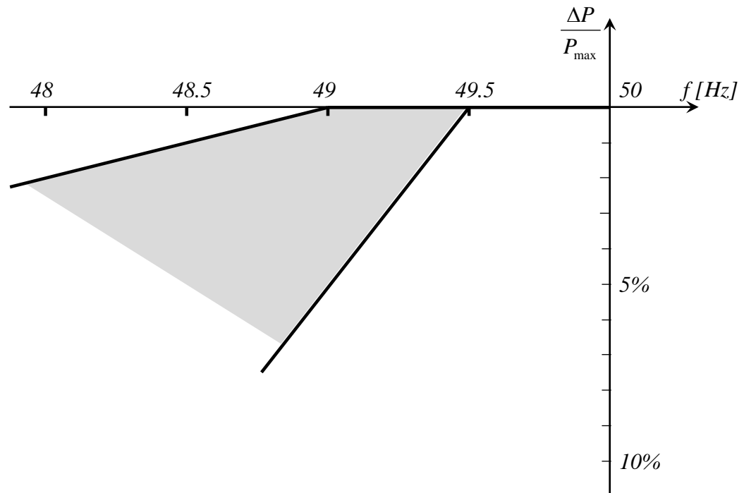
Figure 2: Maximum power capability reduction with falling frequency. The diagram represents the boundaries specified by the relevant TSO.
