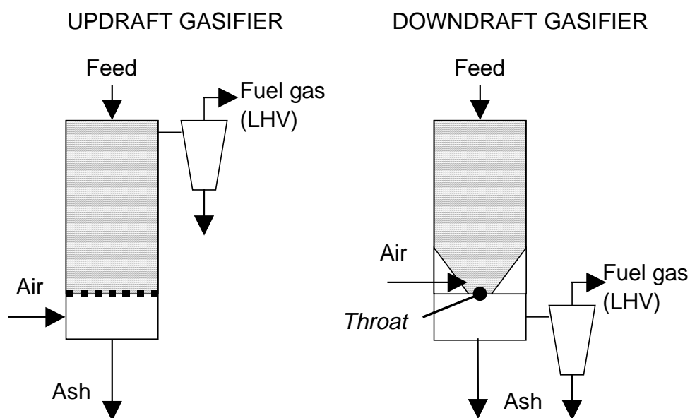
Figure 1 Fixed Bed Gasifiers: Updraft and Downdraft
