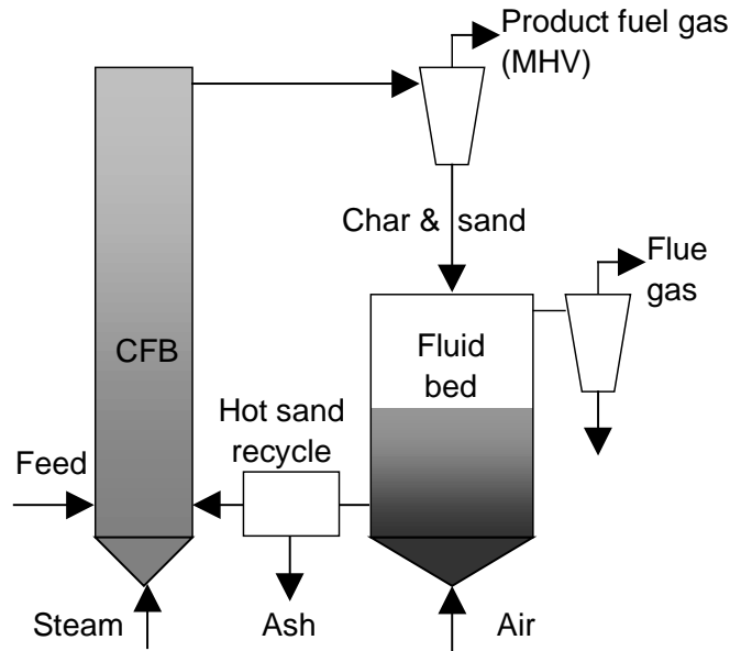
Figure 3 Twin Fluid Bed Gasifier
