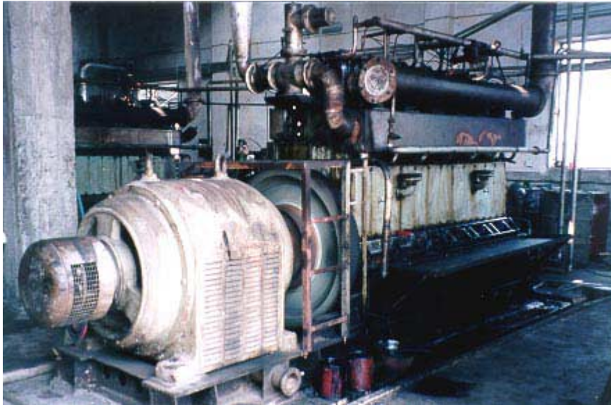
Figure 11 220 kW engine running on LHV gas from rice husk gasification
