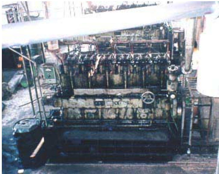
Figure 9 160 kW engines running on LHV gas from rice husk gasification
