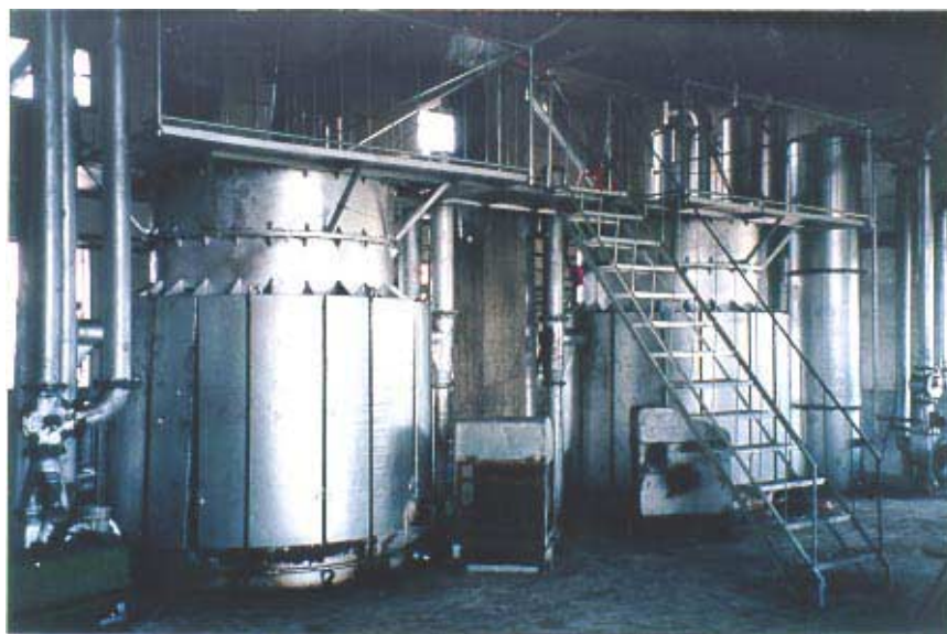
Figure 8 Open core downdraft gasifiers running on rice husks
