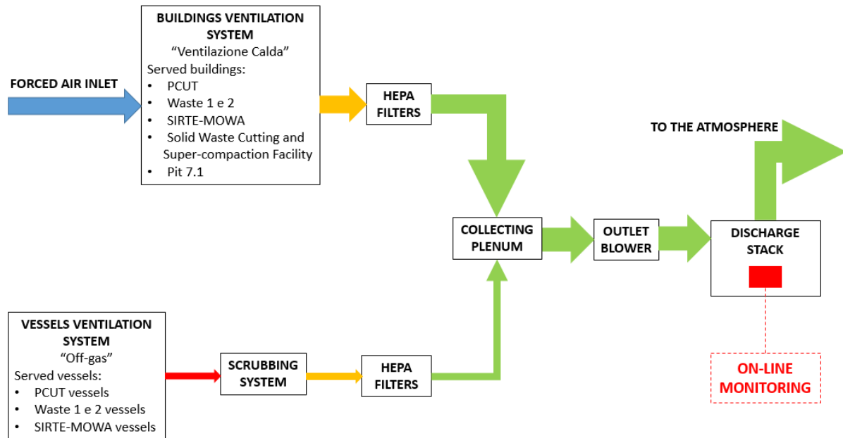
Figure 1. Ventilation system conceptual diagram
