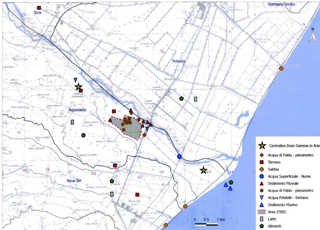
Figure 11. ARPAB monitoring locations in the surroundings of the ITREC facility
