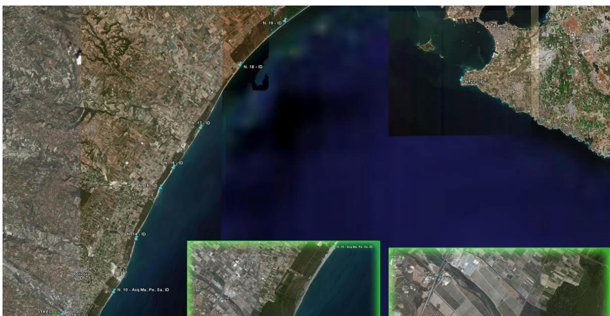
Figure 4. Liquid effluent control points
