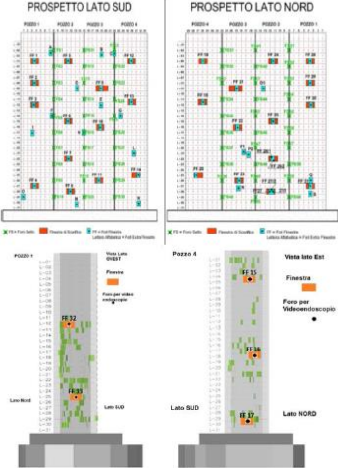
Figure 8. Scheme of the realised drilling holes
