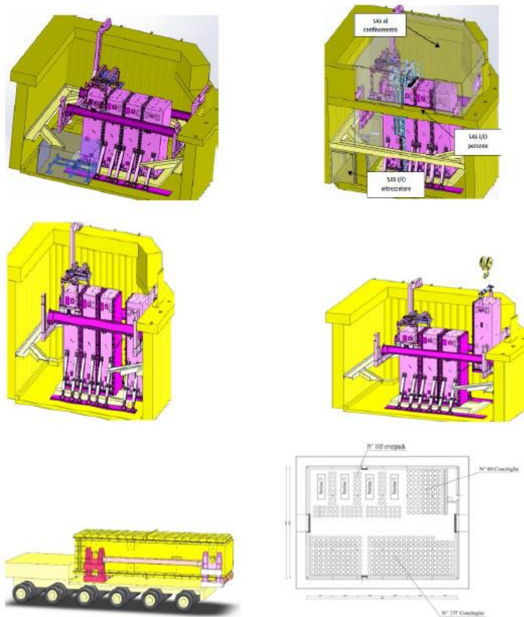
Figure 9. Cutting, lifting and transport of the wells
