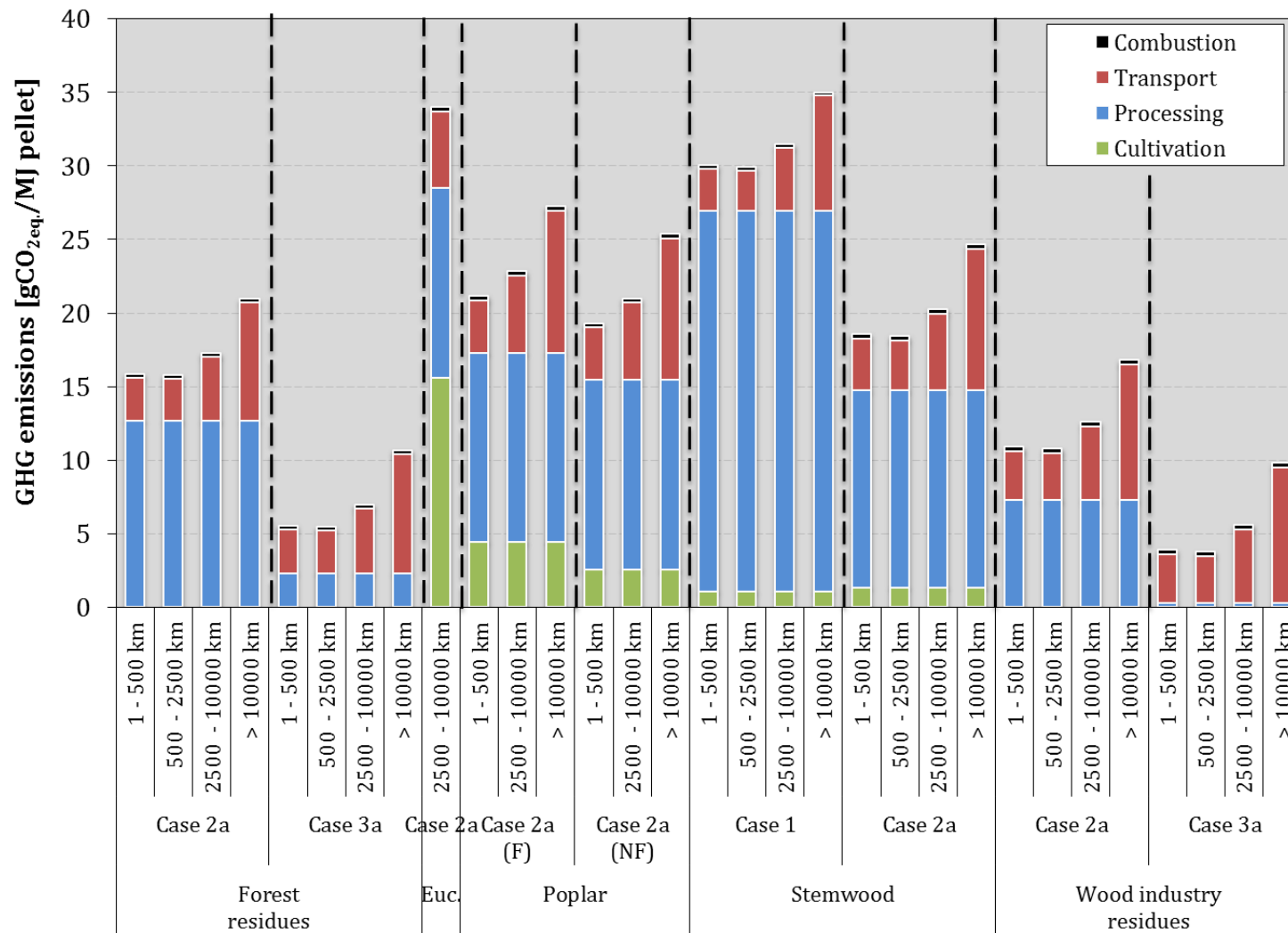
Figure 4: GHG emissions (based on the default values reported in Table 87, Table 88, Table 91 and Table 92) for the most relevant wood pellets pathways. The contribution of the emissions from various steps in the supply chain is also shown in the figure.
